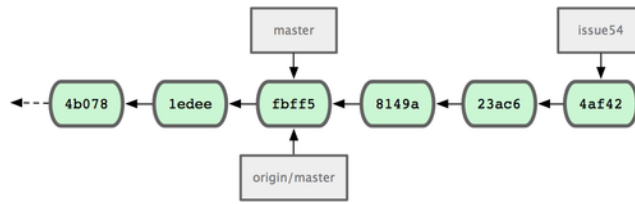
Figure 5.7: Jessica's initial commit history.
